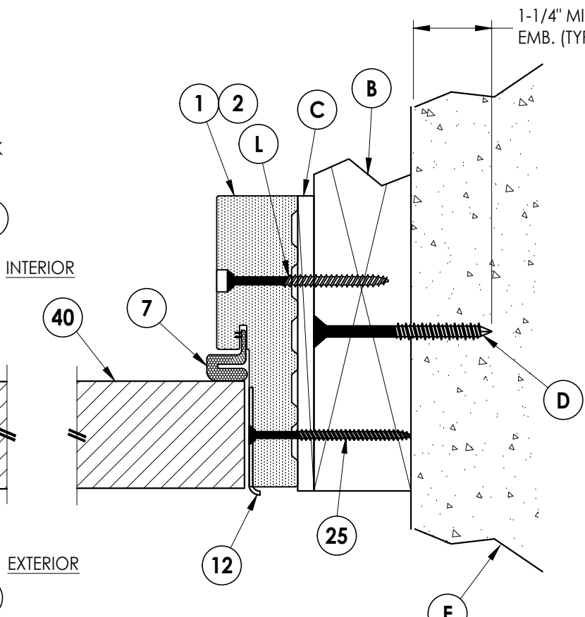
2 6 HORIZONTAL CROSS SECTION Outswing Shown (Inswing Similar) Shown w/ 2X Buck
