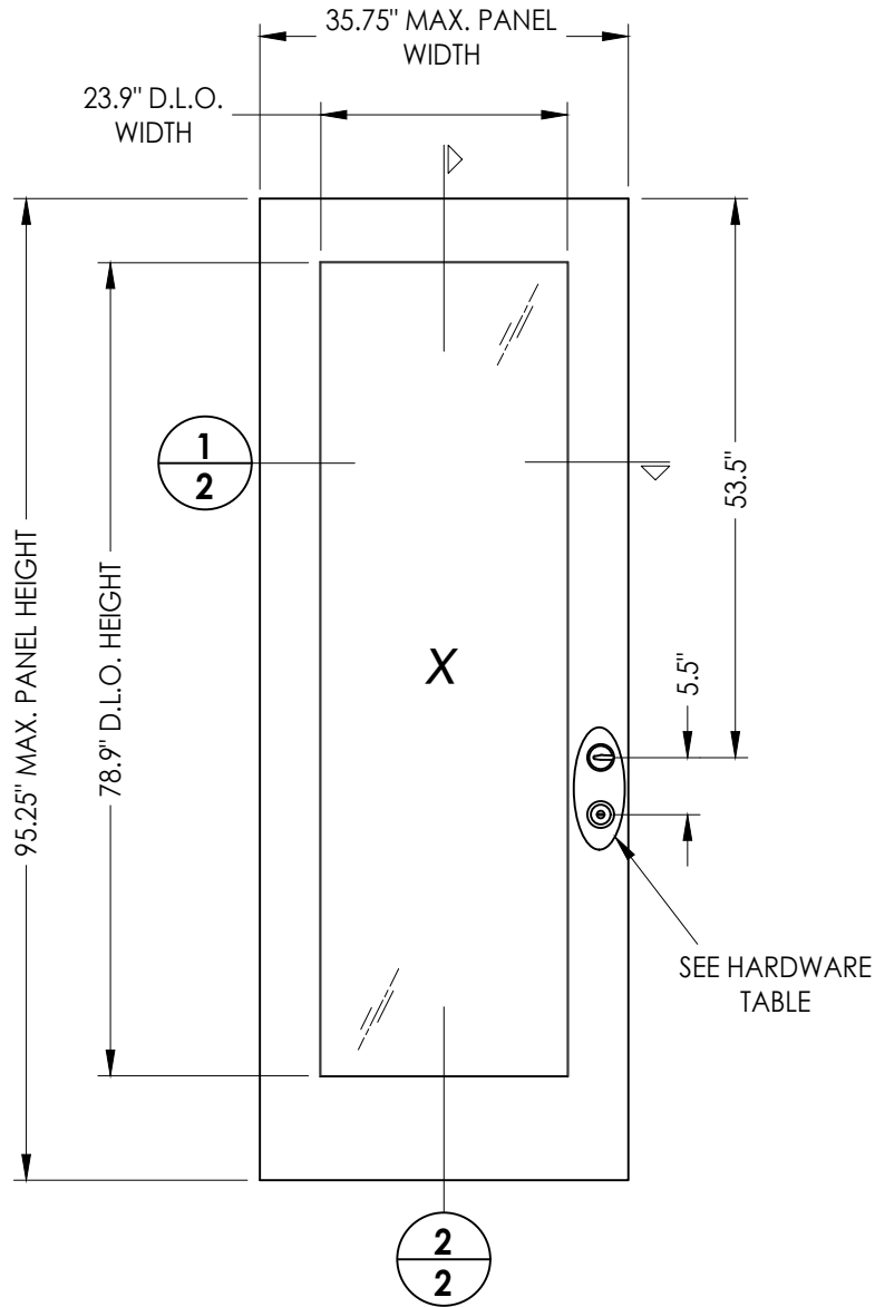
40 FIBERGLASS DOOR PANEL ODL FLUSH GLAZED
